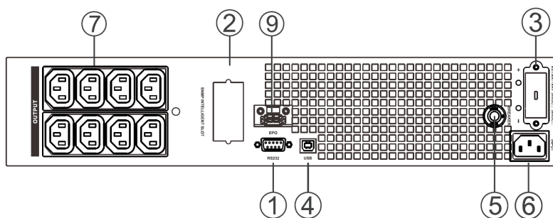
Monolith B 1000RM, 1000RLT, 2000RT
