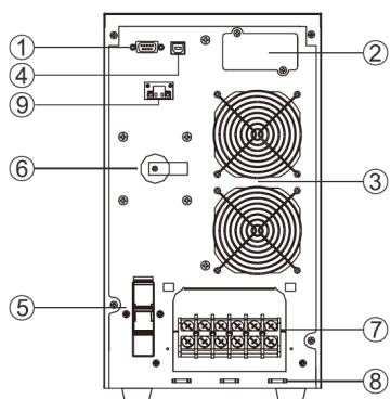
Monolith B 6000LT/10000LT
