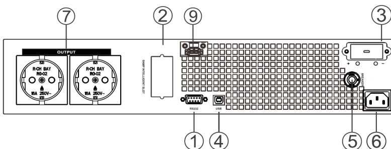
Monolith B 2000RTLT
