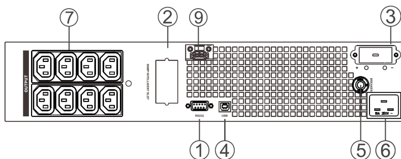
Monolith B 3000RT
